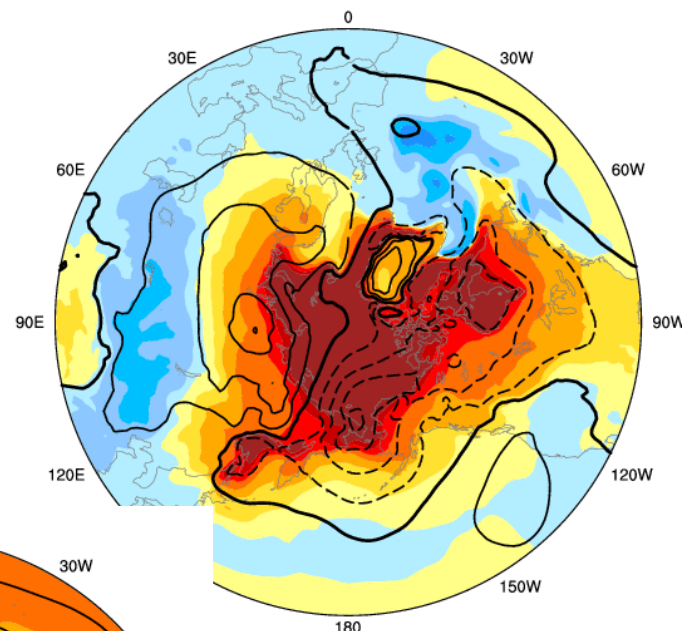
CCSM4-1degree Coupled Ocean-Atmosphere Model
