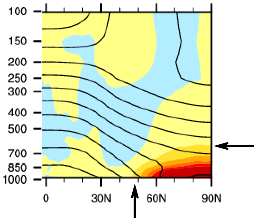
CAM4-1degree Atmospheric Model
