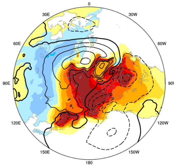
CAM4-1degree Atmospheric Model
