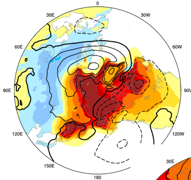
CAM4-1degree Atmospheric Model
