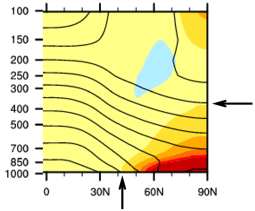
CCSM4-1degree Coupled Ocean-Atmosphere Model
